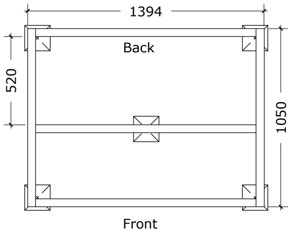
Base frame and recommended support positions.
