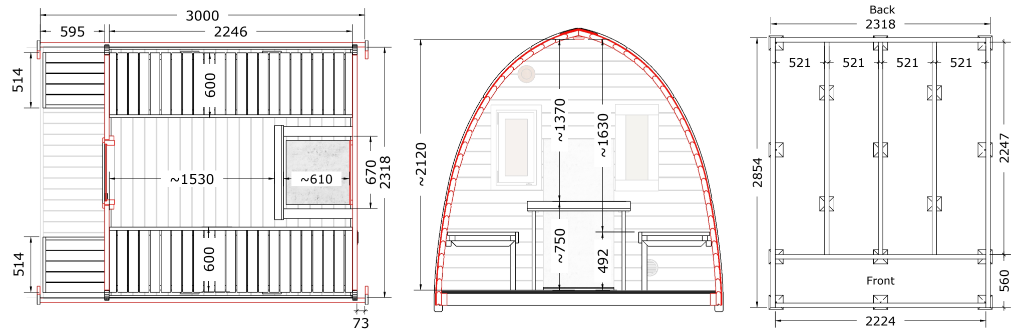
Base frame and recommended support positions
